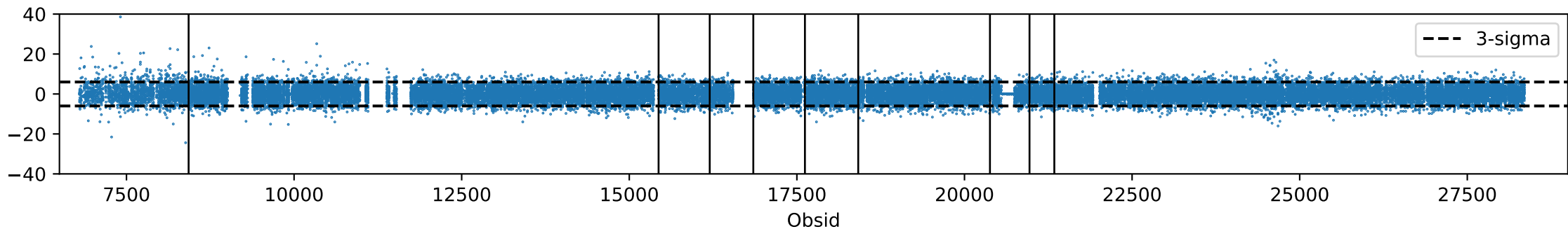
co6, feed 03, PCA mode 4
