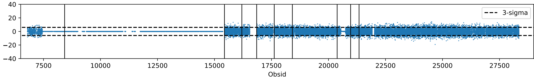
co6, feed 04, PCA mode 3
