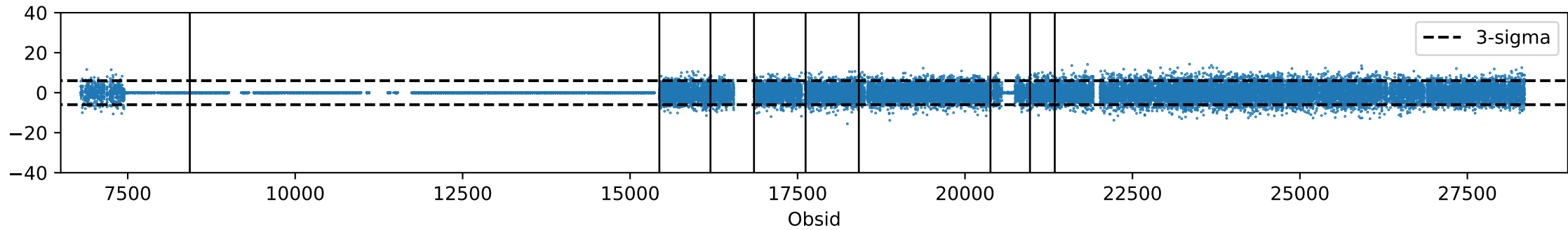
co6, feed 04, PCA mode 6
