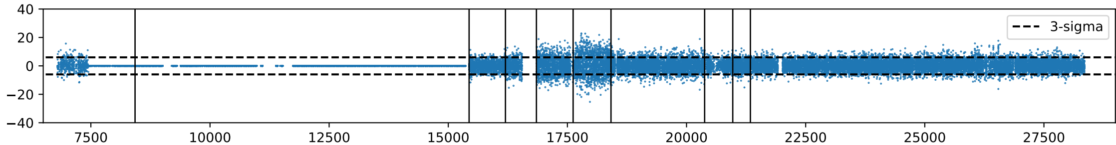
co6, feed 07, PCA mode 1
