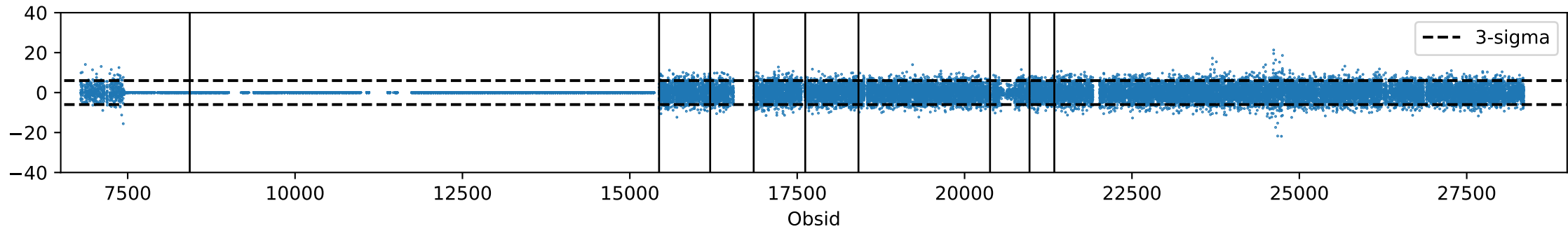
co6, feed 07, PCA mode 6
