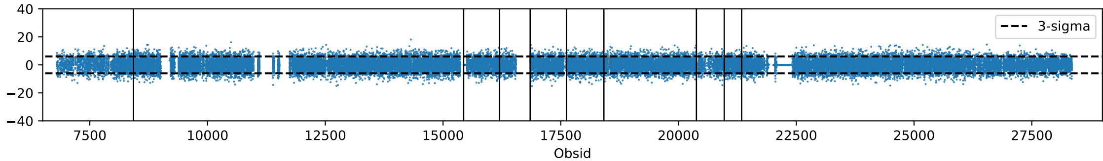
co6, feed 10, PCA mode 4
