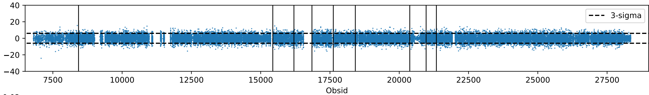
co6, feed 15, PCA mode 3
