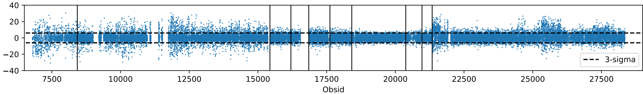
co6, feed 16, PCA mode 2
