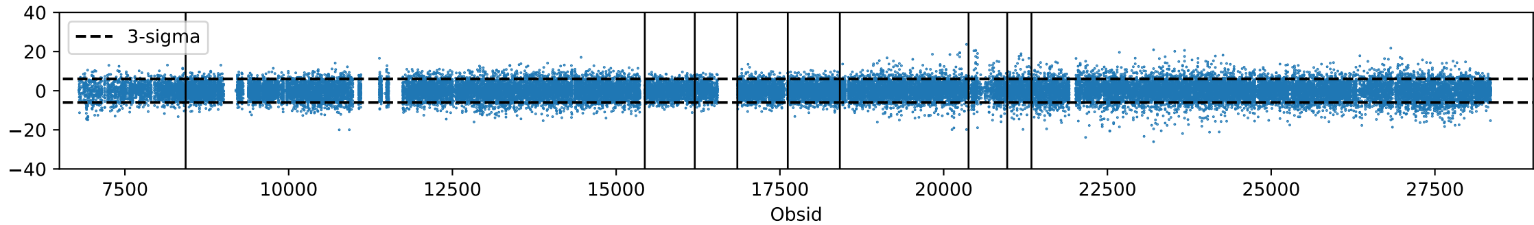
co6, feed 16, PCA mode 3
