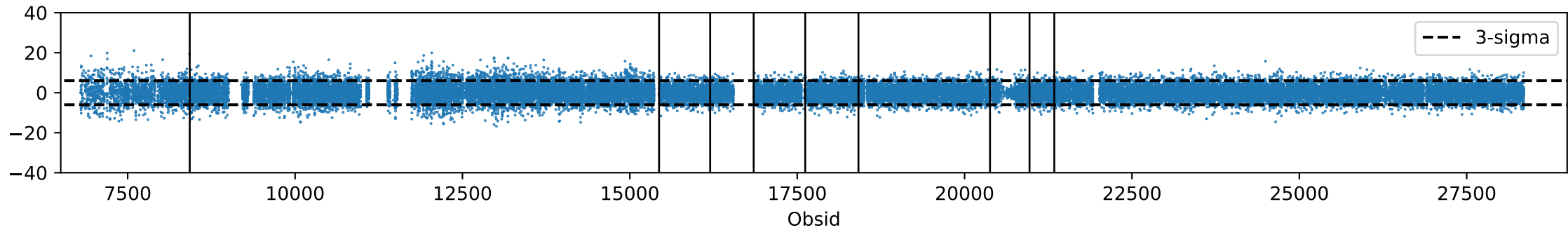
co6, feed 17, PCA mode 5
