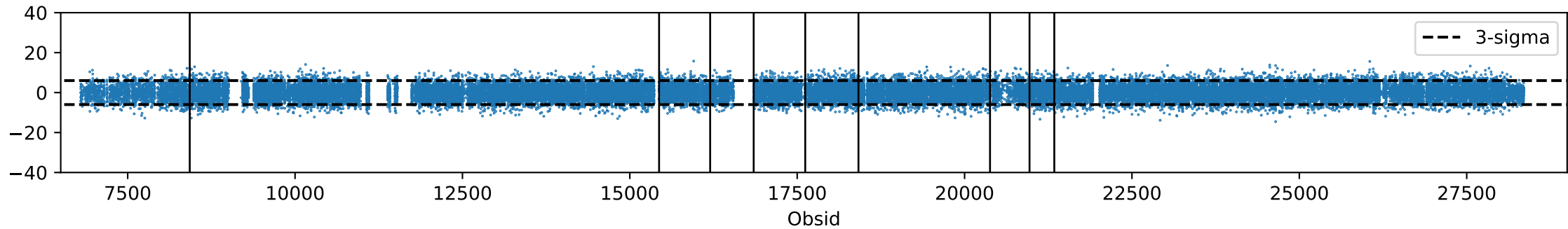
co6, feed 19, PCA mode 5
