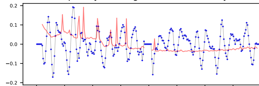
Frequency unit eigen-vector, with Tsys
