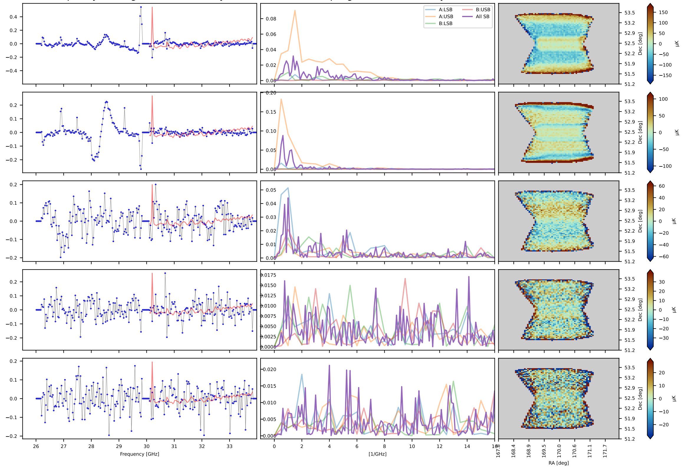
Frequency unit eigen-vector, with Tsys
