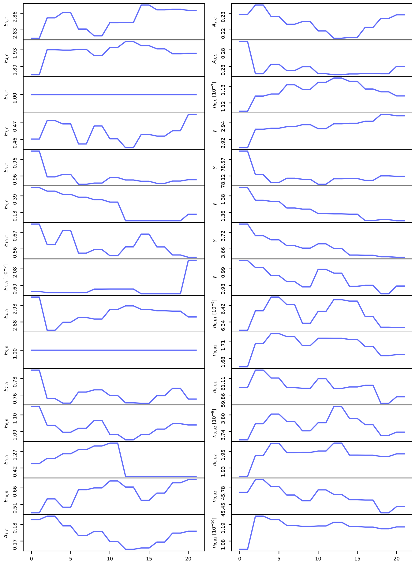
Gibbs iteration
